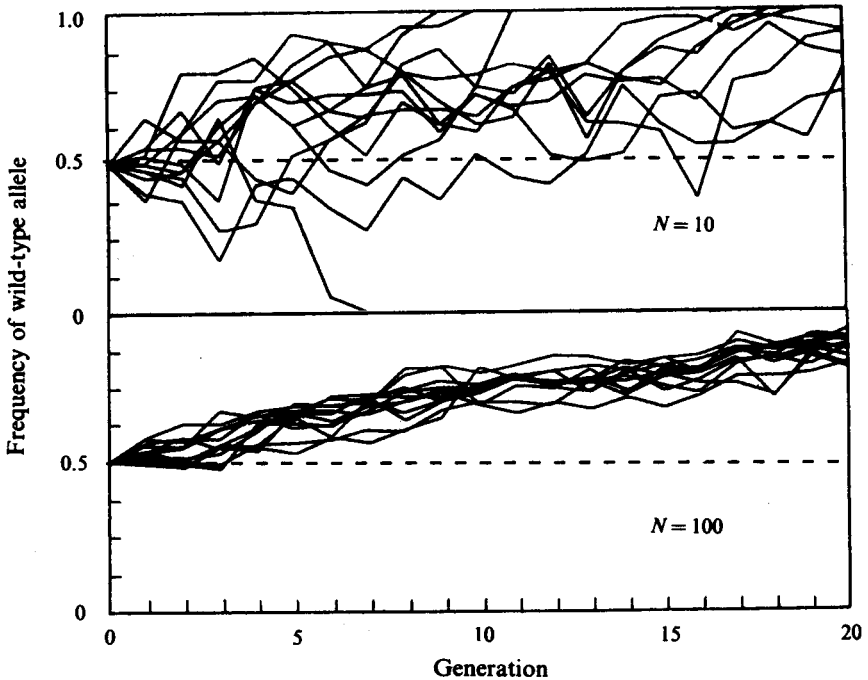
Fig. 3.2. Random drift of a colour gene ('black') in Tribolium . Heterozygotes were recognizable, so the gene frequencies were estimated exactly by counting. The figure shows the results with two population sizes, N = 10 and N = 100 . There were 12 lines with each population size. Natural selection favoured the wild-type allele and led to an overall increase in its frequency, random drift causing variation of the lines around the mean, more marked in the smaller than in the larger populations. (After Rich, Bell, and Wilson, 1979.)
