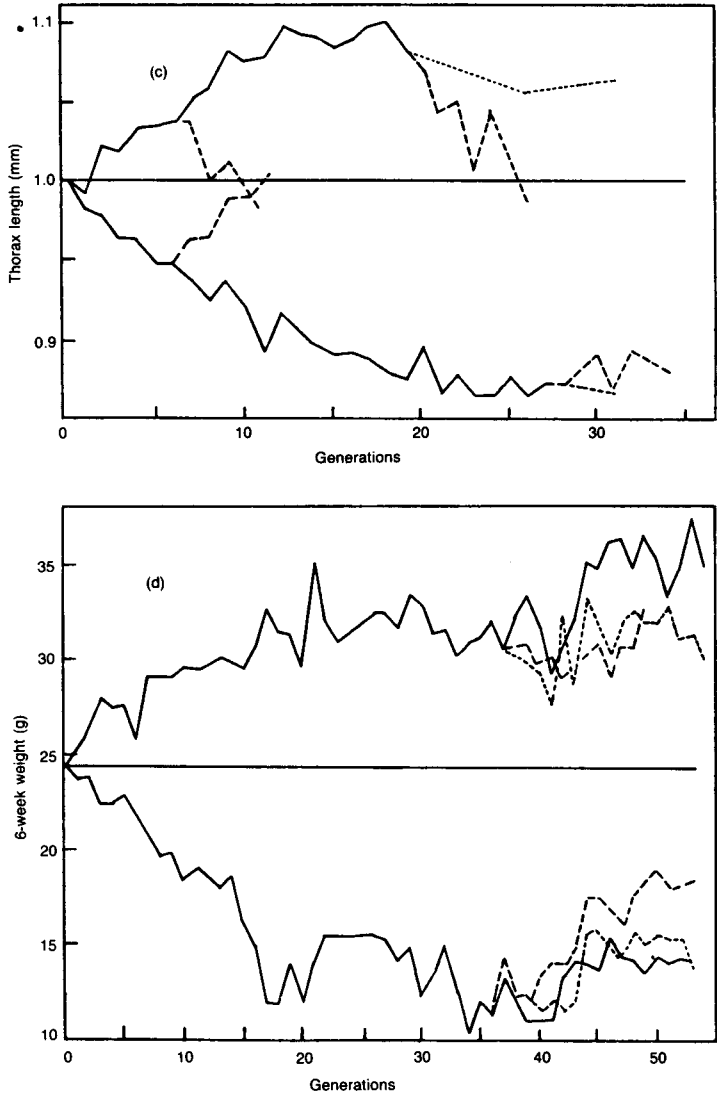
(c) Drosophila melanogaster , thorax length. (After F. W. Robertson, 1955.)
