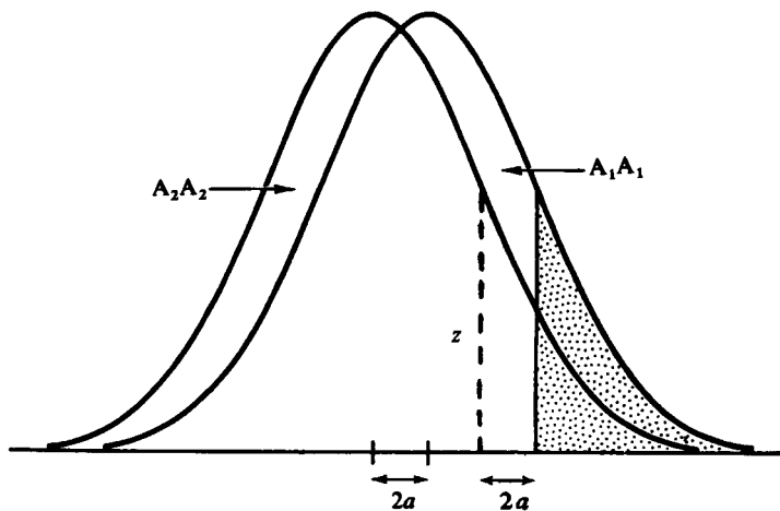
Fig. 11.6. Selection for a metric character operating on one of the loci concerned.
