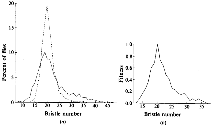
Fig. 20.3. (a) Distributions of sternopleural bristle number in Drosophila : continuous line, under weak natural selection; broken line, under strong natural selection. (b) Fitness profile derived from the frequency distributions in (a). The fitness scale is relative to the fittest bristle class. The fitness measured is only the component, survival from egg to adult, and not the whole of fitness. (Adapted from Kearsy and Barnes, 1970.)
