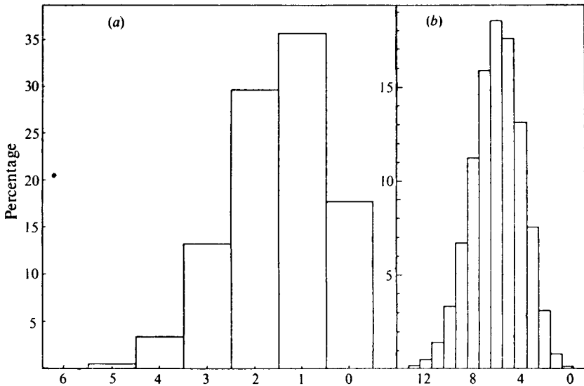
Fig. 6.1. Distributions expected from the simultaneous segregation of two alleles at each of several or many loci: (a) 6 loci, (b) 24 loci. There is complete dominance of one allele over the other at each locus, and the gene frequencies are all 0.5. Each locus, when homozygous for the recessive allele, is supposed to reduce the measurement by 1 unit in (a), and by \frac{1}{4} unit in (b). The horizontal scale, representing the measurement, shows the number of loci homozygous for the recessive allele, and the vertical axis shows the probability, or the percentage of individuals expected in each class. The probabilities are derived from the binomial expansion of (\frac{1}{2} + \frac{1}{2})^n , where n is the number of loci.
