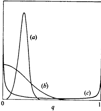
Fig. 4.2. Theoretical distributions of gene frequency among sub-populations when the dispersion is balanced by mutation and selection. The graphs refer to a recessive gene with u = v = \frac{1}{20}s , in populations of size: (a) N_e = 50/s , (b) N_e = 5/s , and (c) N_e = 0.5/s . (Based on Wright, 1942.)
