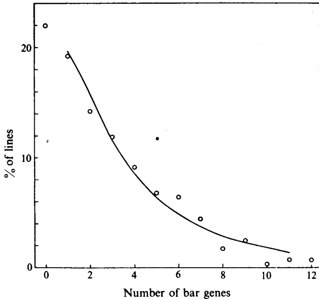
Fig. 4.3. Distribution of gene frequencies under inbreeding and selection, as explained in Example 4.2. (Data from Wright and Kerr, 1954.)
