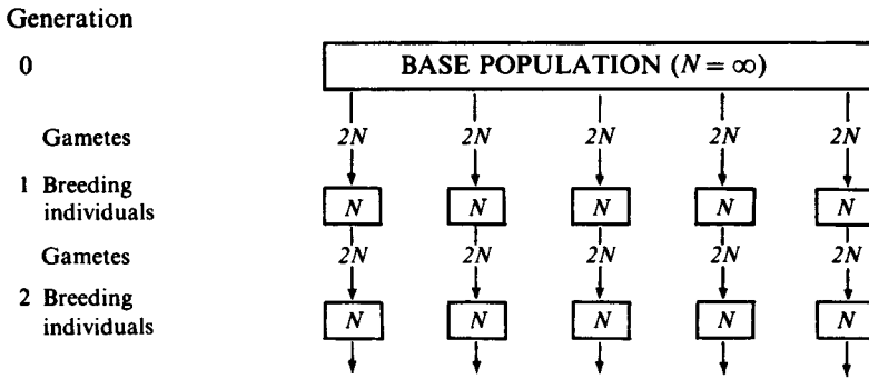
Fig. 3.1. Diagrammatic representation of the subdivision of a single large population – the base population – into a number of sub-populations, or lines.
