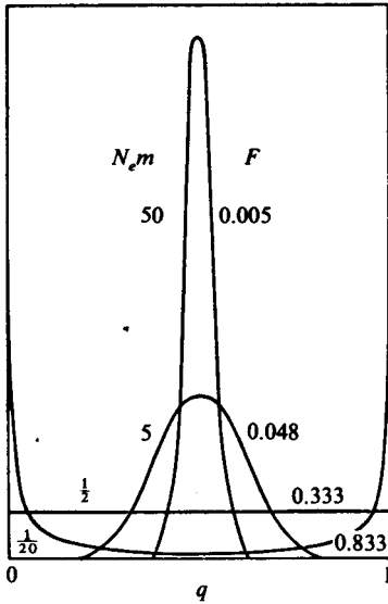
Fig. 4.1. Theoretical distributions of gene frequency among sub-populations, when dispersion is balanced against mutation or migration, and the mean gene frequency is 0.5. The vertical axis is the probability, as in Fig. 3.5. The states of dispersion to which the curves refer are indicated by the values of F in the figure. The values of N_e m are the numbers of immigrants per generation, as explained in the text. (Based on Wright, 1951.)
