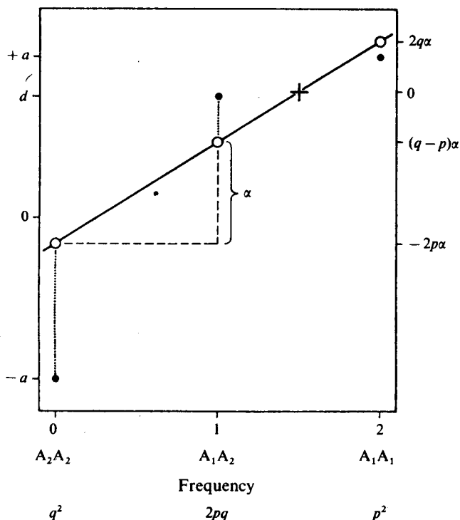
Fig. 7.2. Graphical representation of genotypic values (closed circles), and breeding values (open circles), of the genotypes for a locus with two alleles, A_1 and A_2 , at frequencies p and q , as explained in the text. Horizontal scale: number of A_1 genes in the genotype. Vertical scales of value: on left – arbitrary values assigned as in Fig. 7.1; on right – deviations from the population mean. The figure is drawn to scale for the values: d = \frac{3}{4}a , and q = \frac{1}{4} .
