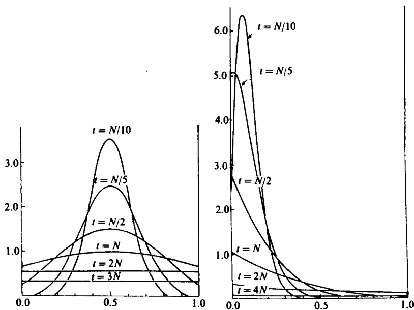
Fig. 3.5. Theoretical distributions of gene frequencies among lines, after different numbers of generations, t , expressed in terms of the population size of the lines, N . In the left-hand figure q_0 = 0.5 ; on the right q_0 = 0.1 . Previously fixed lines (see next section) are excluded. The horizontal scale is the gene frequency, q , in any line. The vertical axis is the probability, scaled to make the area under each curve equal to the proportion of unfixed lines. (After Kimura, 1955.)
