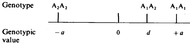
Fig. 7.1. Arbitrarily assigned genotypic values.
