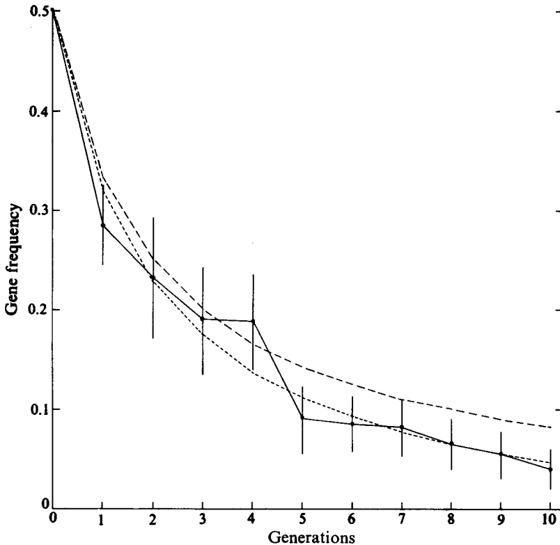
Fig. 2.4. Change of gene frequency under natural selection in the laboratory, as described in Example 2.1. (Adapted from Wallace, 1963.)
